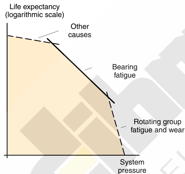
Hydraulic unit life versus system pressure.
