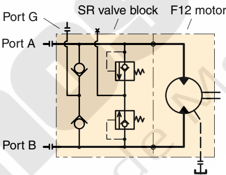
SR valve block schematic.
