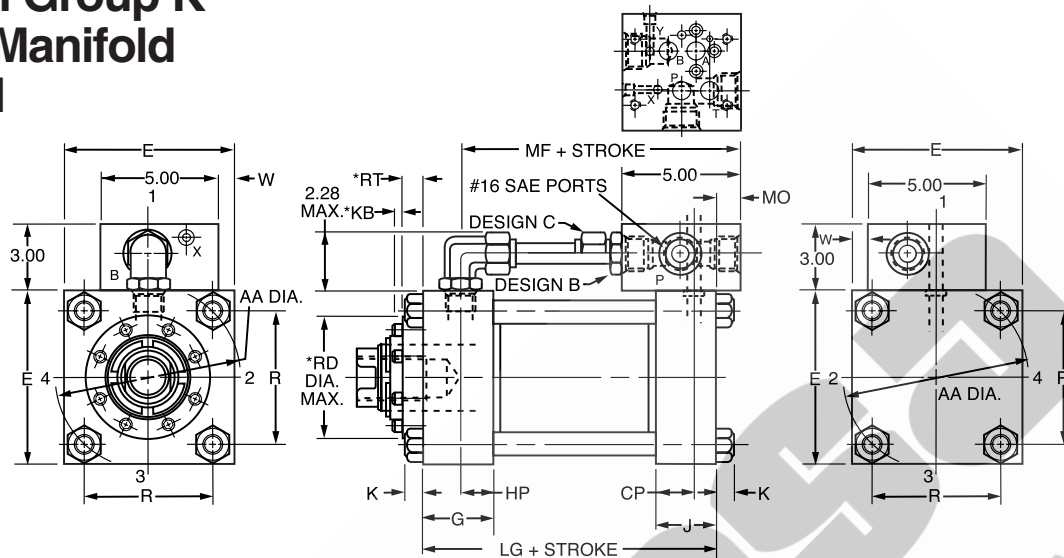
Group K/NFPA D07 Valve Manifold, Cap End Mounted Series 3HX Cylinder
