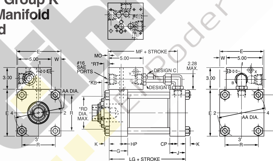
Group K/NFPA D07 Valve Bolt-on Manifold, Head End Mounted, Series 3HX Cylinder
