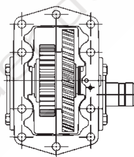
Assembly Arrangement 4*
