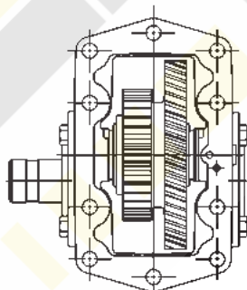
Assembly Arrangement 5**
