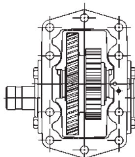
Assembly Arrangement 6*
