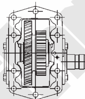
Assembly Arrangement 3
