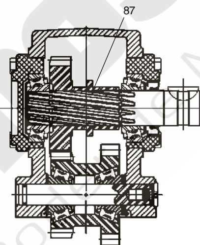
447 Series Ass'y 4 &amp; 6
