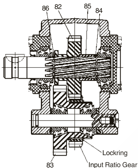
442 &amp; 489 Series Ass'y 4 &amp; 6
