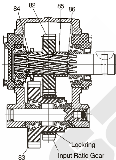
442 &amp; 489 Series Ass'y 3 &amp; 5
