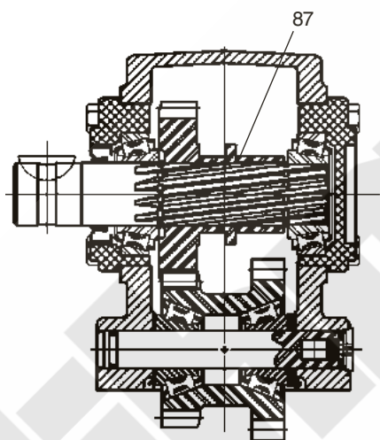
447 Series Ass'y 3 &amp; 5
