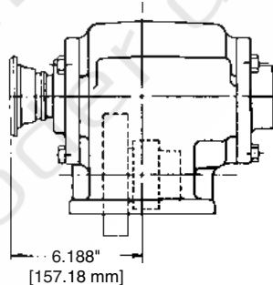
Assembly 6
