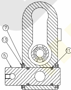
30 GPM ROTOR
