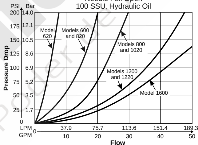
Controlled Flow vs. Pressure Drop Needle Full Open 100 SSU, Hydraulic Oil
