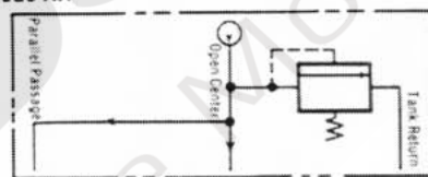
typical schematic
