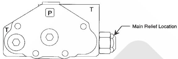
No. 23613 Inlet Cover for all Non-Solenoid Valves
