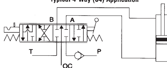
Typical 4-Way Float (K4) Application
