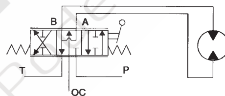
Typical 4-Way Free Flow (F4) Application
